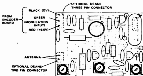
FIGURE I RF DECK WIRING
