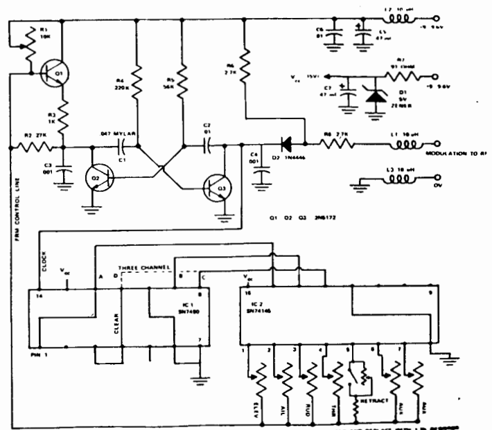
ENCODER SCHEMATIC
