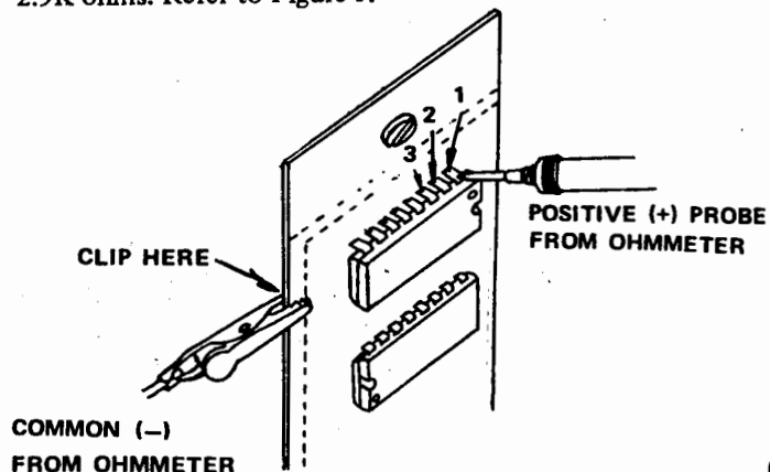
FIGURE J TEST POINTS
