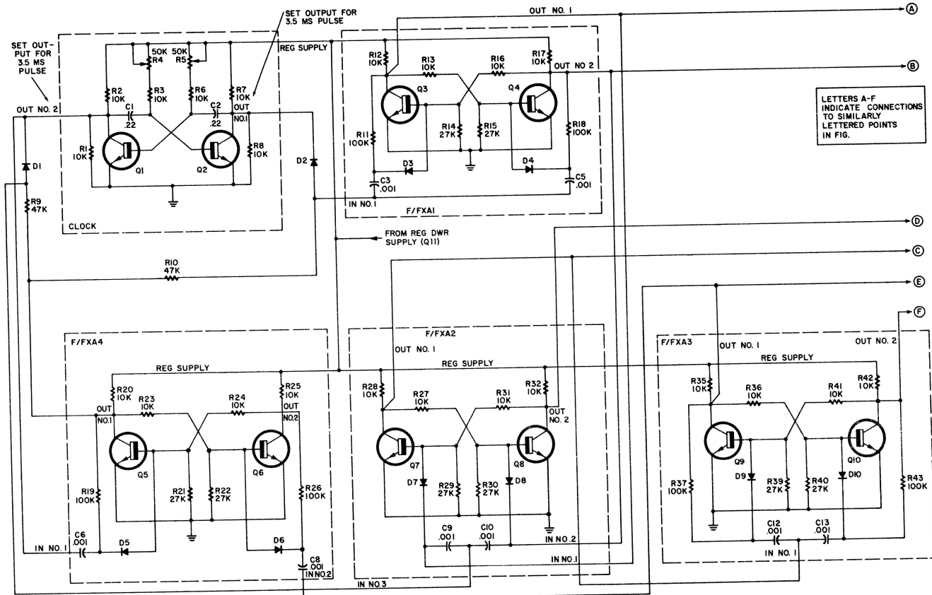
Bonner Digimite 8 transmitter part 2
